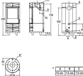
Model: ROUND BCS
