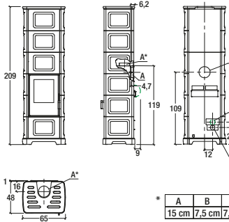
Model: E928 C-H BCS
