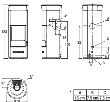
Model: E929 T BCS
