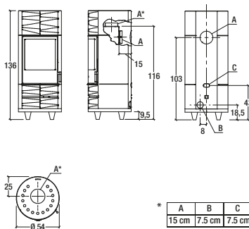
Model: ROUND-M Hermetic
