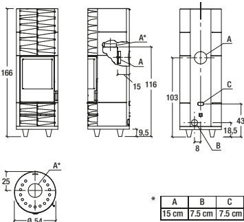
Model: ROUND-H Hermetic
