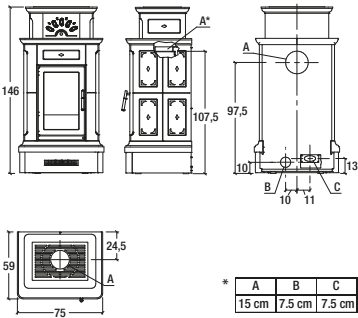
Model: CANAZEI BCS
