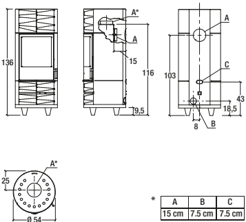
Model: ROUND-M BCS
