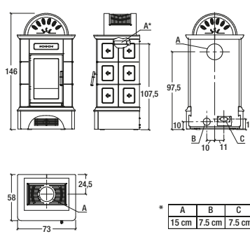
Model: BRUNICO BCS
