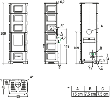
Model: E928 C-H BCS
