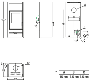
Model: E928 BCS
