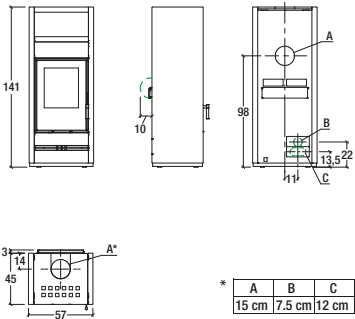
Model: E928 S
