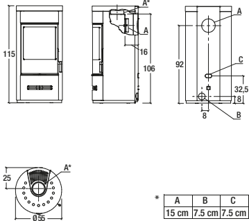
Model: E929 M Hermetic
