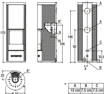
Model: E929 D-H Hermetic
