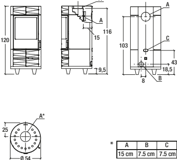
Model: ROUND Hermetic
