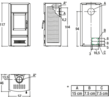
Model: E927 D BCS
