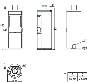
Model: E924 A Hermetic
