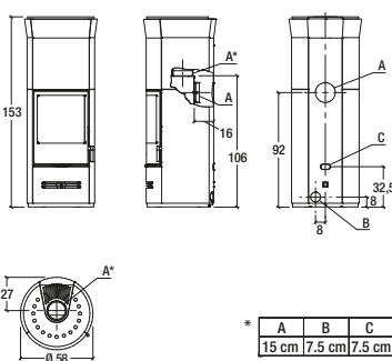
Model: E929 T Hermetic
