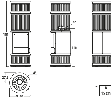
Model: E929 C-H BCS
