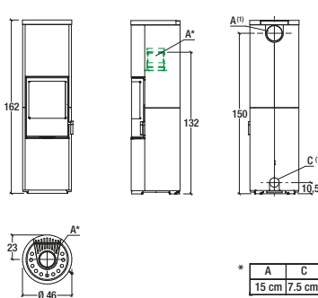
Model: E924 A-H Hermetic
