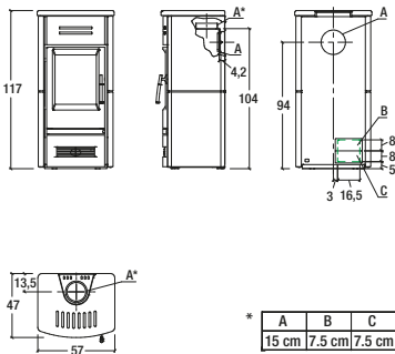
Model: E927 M
