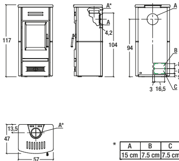
Model: E927 M BCS
