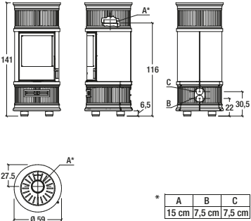
Model: E929 C Hermetic
