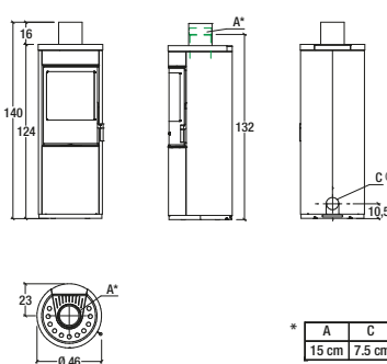
Model: E924 A BCS
