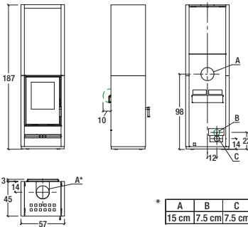
Model: E928-H BCS
