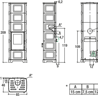
Model: E928 C-H
