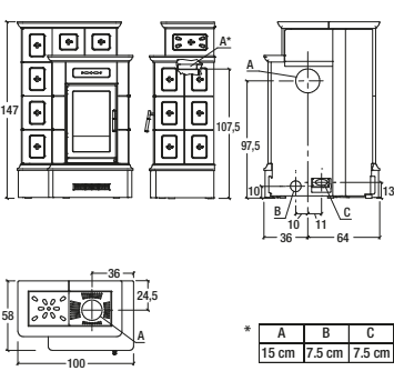
Model: ORTISEI BCS
