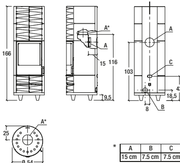
Model: ROUND-H BCS
