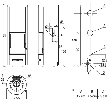
Model: E929 M-H Hermetic
