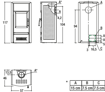
Model: E927 D
