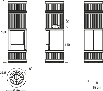
Model: E929 C-H Hermetic
