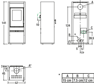
Model: E928 A
