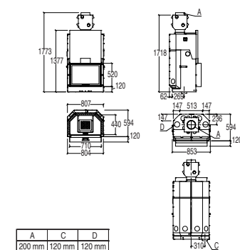
ME 70 WITH HOOD COVER (to be mounted during installation phase)
