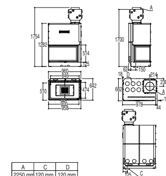
MA 283 D/S SL PLUS INCL. VENTILATION MANTLE KIT (to be mounted during installation phase)
