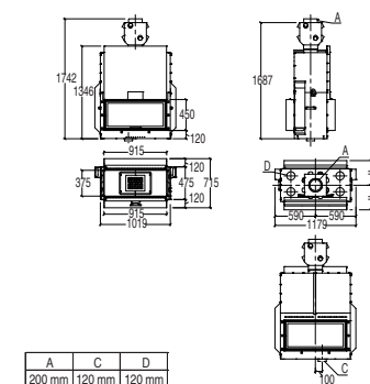
ME 90 WITH HOOD COVER (to be mounted during installation phase)
