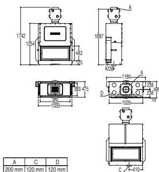
MA 263 B SL PLUS INCL. VENTILATION MANTLE KIT (to be mounted during installation phase)
