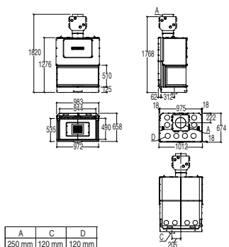
MA 271 SL PLUS INCL. VENTILATION MANTLE KIT (to be mounted during installation phase)
